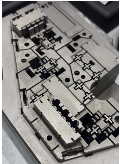
After 400,000 shots
